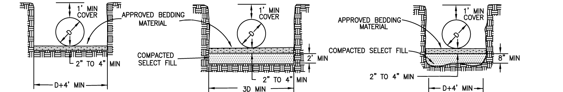
BEDDING OF CULVERTS ON STABLE NATURAL GROUND FOUNDATION BEDDING OF CULVERTS ON SOFT SPONGY, UNSTABLE SOIL FOUNDATION OR COMPACTED EMBANKMENT BEDDING OF CULVERTS IN SOLID ROCK OR BOULDER FOUNDATION
