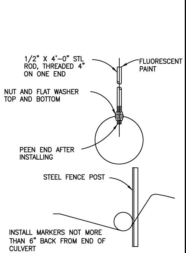
CULVERT MARKER INSTALLATION
