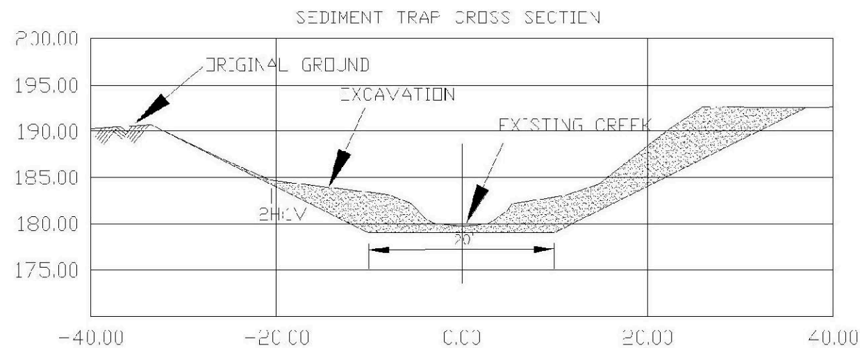
TYPICAL SEDIMENT TRAP CROSS-SECTION NTS (12) X
