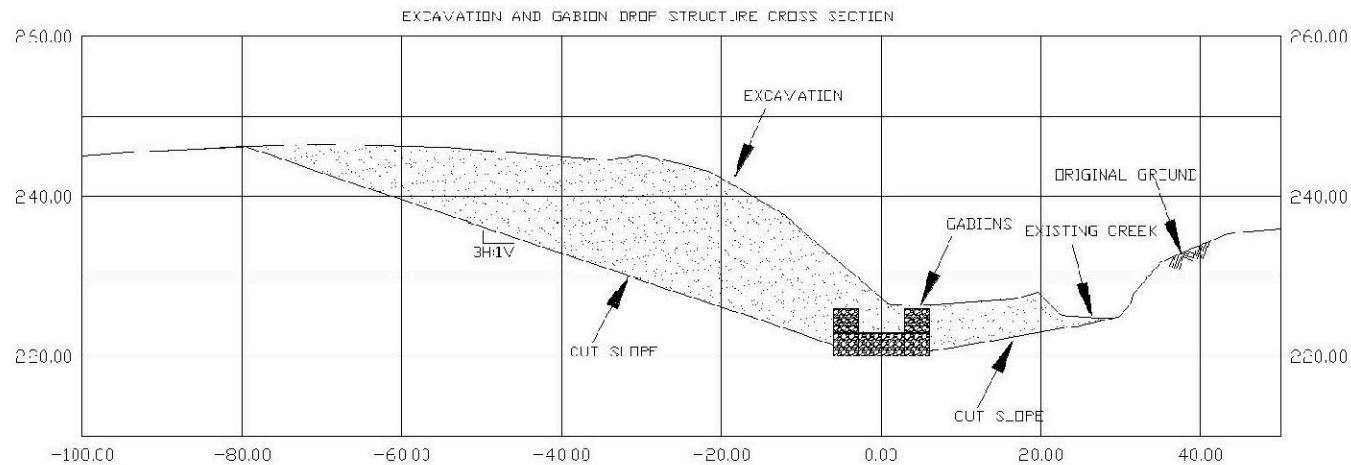
TYPICAL GABION DROP STRUCTURE NTS (10) X
