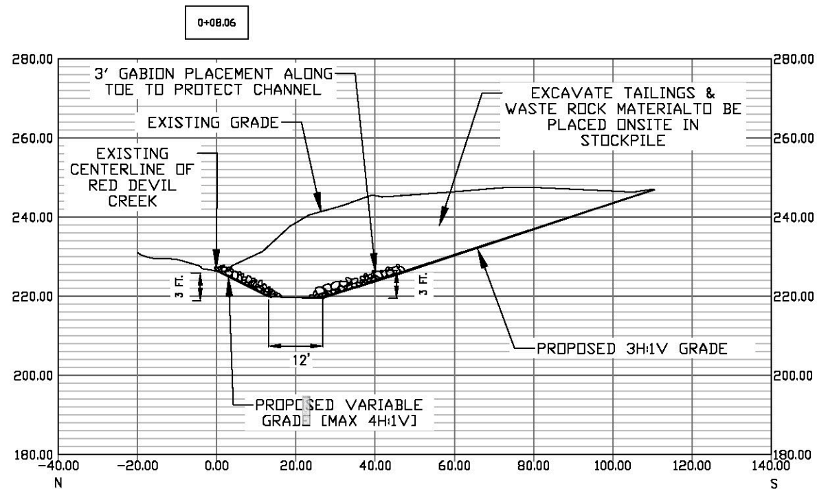
TYPICAL CROSS-SECTION EXCAVATION CHANNEL NTS (9) X
